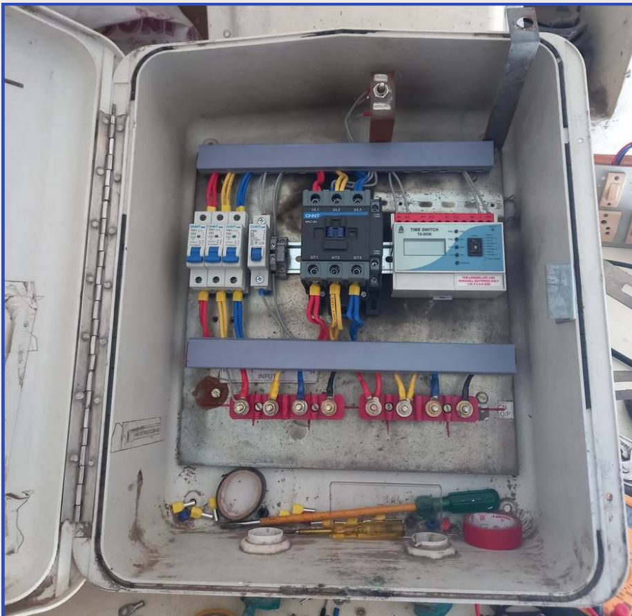
DOL/STAR-DELTA PANEL
